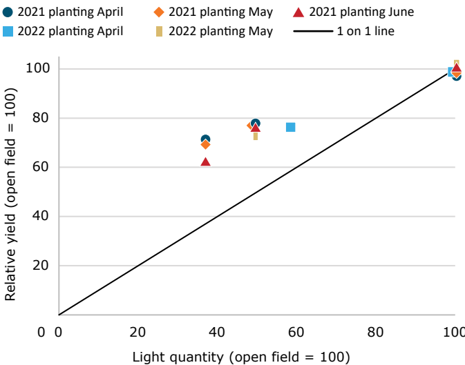
Figure 5 Above: growing strawberries under a partially transparent solar cover, Groenleven system (photo: Herman Helsen). Below: Relative strawberry production as a function of transmittance of the solar roof cover (both relative to open field production). At 60% light permeability of the system, crops receive 40% less light than in the open field. Strawberry production is then 75% of that in the open field.
